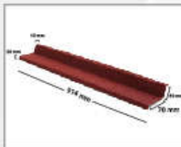
WALL FLASHING
