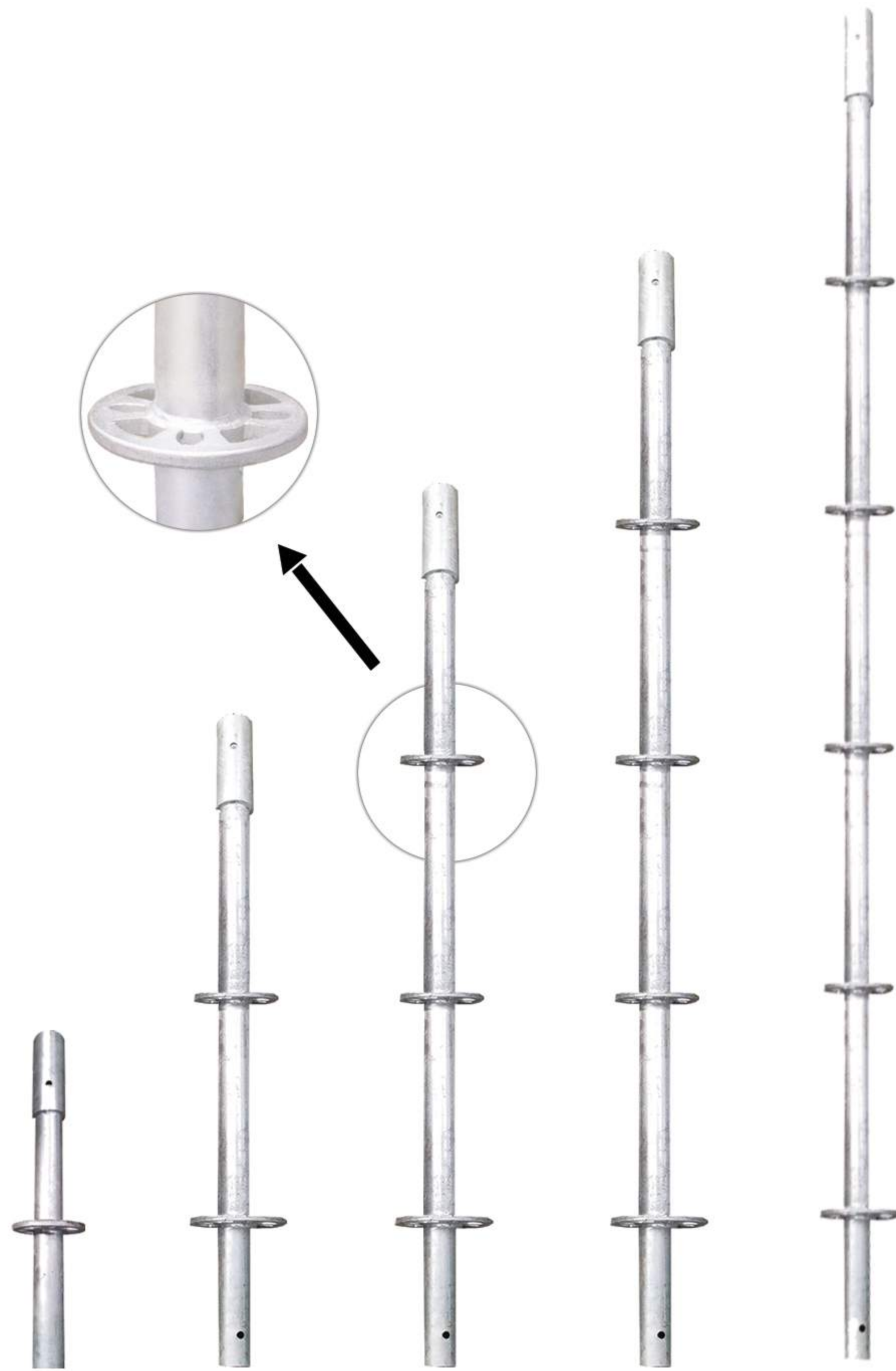
RINGLOCK STANDARD
