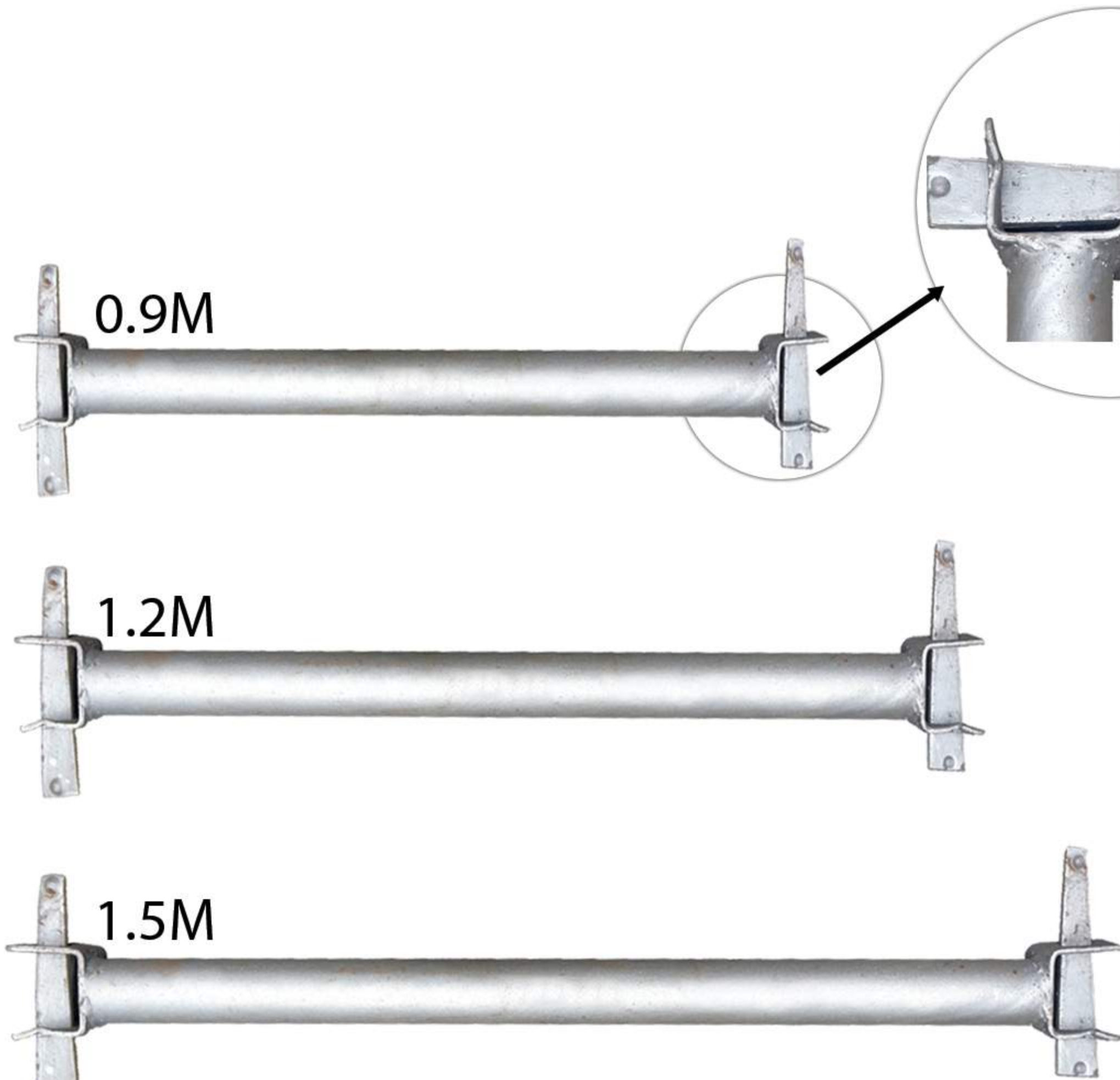
LEDGER
