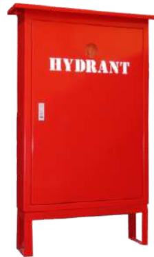
Type C Size: 66x95x20 Cm
