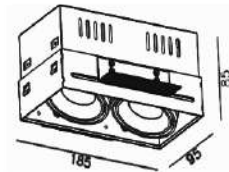
Type Cut Hole FR 1055 B-L 183 x 96
